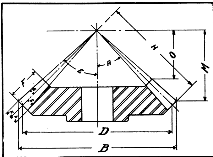
Fig. 20—Diagram of a miter gear for use in connection with formulæ of the same.
